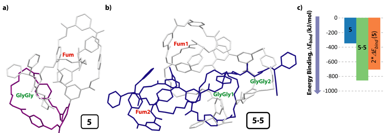
Fig. 5 Computational models at DFT level in \text{CHCl}_3 (BP86–D3/def2–SVP) of: (a) [2]rotaxane 5 ; (b) cyclic hetero[4]pseudorotaxane (dimer 5 · 5 ); (c) diagram for visually comparing the binding energies of the monomer 5 , the cooperatively self-assembled dimer 5 · 5 and that of the double of binding energy of the monomer 5 . Both calculated structures are the lowest energy ones; \Delta E_{\text{bind}} : variation of the binding energy calculated as the difference between the energy of the complex minus the energy of all separated molecules that formed it (of the conformer with the lowest energy). For clarity the hydrogen atoms have been removed. Note that in the cyclic dimer 5 · 5 , one of the molecules is colored in grey and the second one in dark blue. For clarity the diamide macrocycle is colored in purple in monomer 5 .
