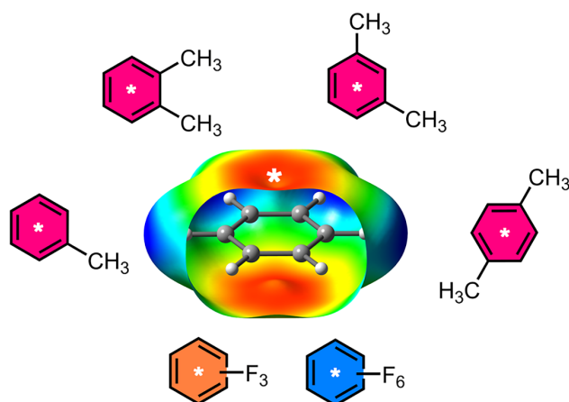
Figure 4. MEP surface of benzene (0.002 a.u.) and schematic representation of the additional VOCs used. The values at the ring centroid (indicated with a white asterisk) as well as the MEP minima and maxima are gathered in Table 1 (kcal/mol).
