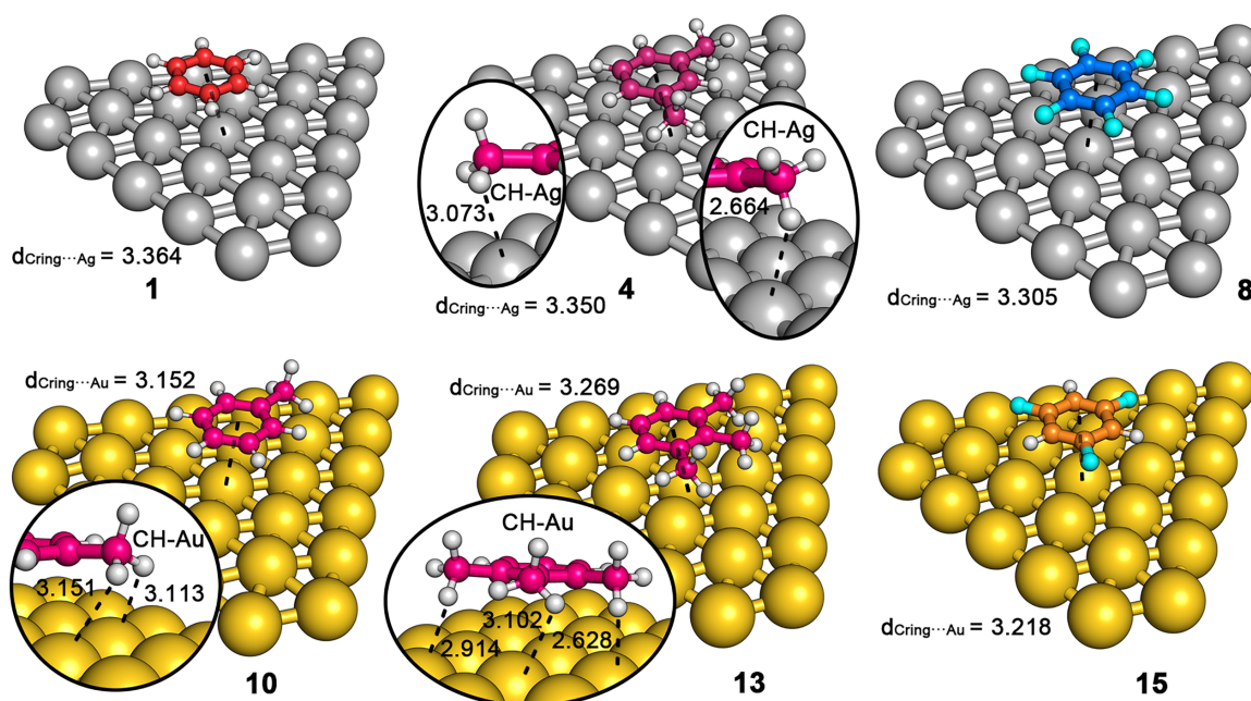
Figure 5. Optimized geometries (PBE0-D3/def2-TZVP level of theory) of complexes 1 , 4 , 8 , 10 , 13 and 15 . Distances ( d_{\text{ring centroid}} \cdots \text{Ag/Au} ) are given in Å. Ancillary CH-Rg interactions are also indicated inside the circular parts of the image.
