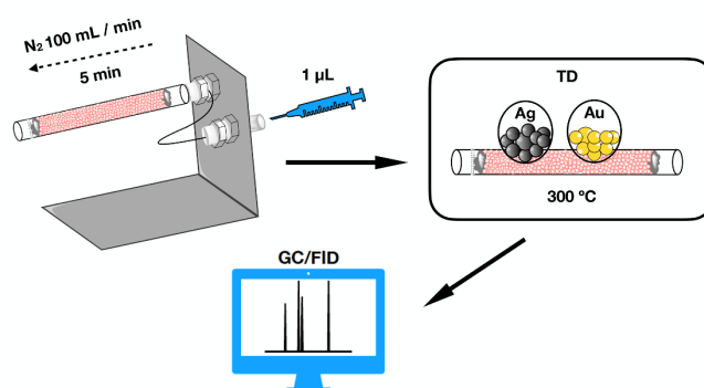
Figure 8. Schematic representation of the analytical procedure.
