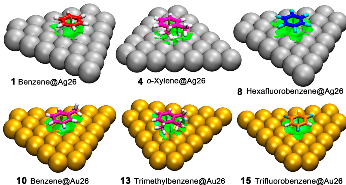
Figure 7. Non Covalent Interaction (NCI) plot analyses of complexes 1 , 4 , 8 , 10 , 13 and 15 . NCIplot color range -0.035 \text{ au} \leq (\text{sign}\lambda_2)\rho \leq +0.035 \text{ au} . Isosurface value |\text{RGD}| = 0.5 and intercut parameter of 0.75.
