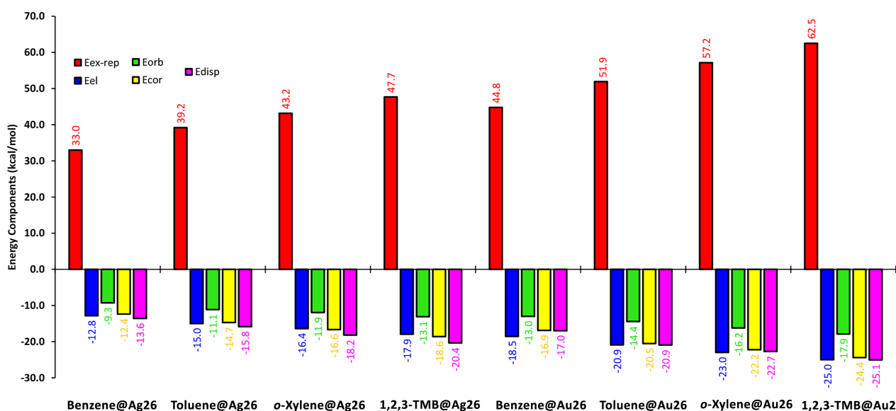
Figure 6. Energy Decomposition Analysis into exchange-repulsion ( E_{\text{ex-rep}} ), electrostatics ( E_{\text{el}} ), orbital ( E_{\text{orb}} ), electron correlation ( E_{\text{cor}} ) and dispersion ( E_{\text{disp}} ) terms in kcal/mol for complexes 1 to 3 , 6 , 9 to 11 and 14 . TMB stands for trimethylbenzene.
