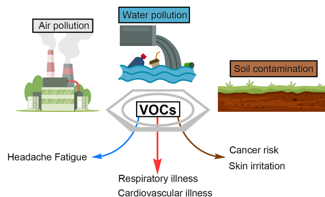
Figure 1. Schematic representation of the VOC accumulation in different environments (air, water, and soil) (top) and their impact in our health (bottom).
