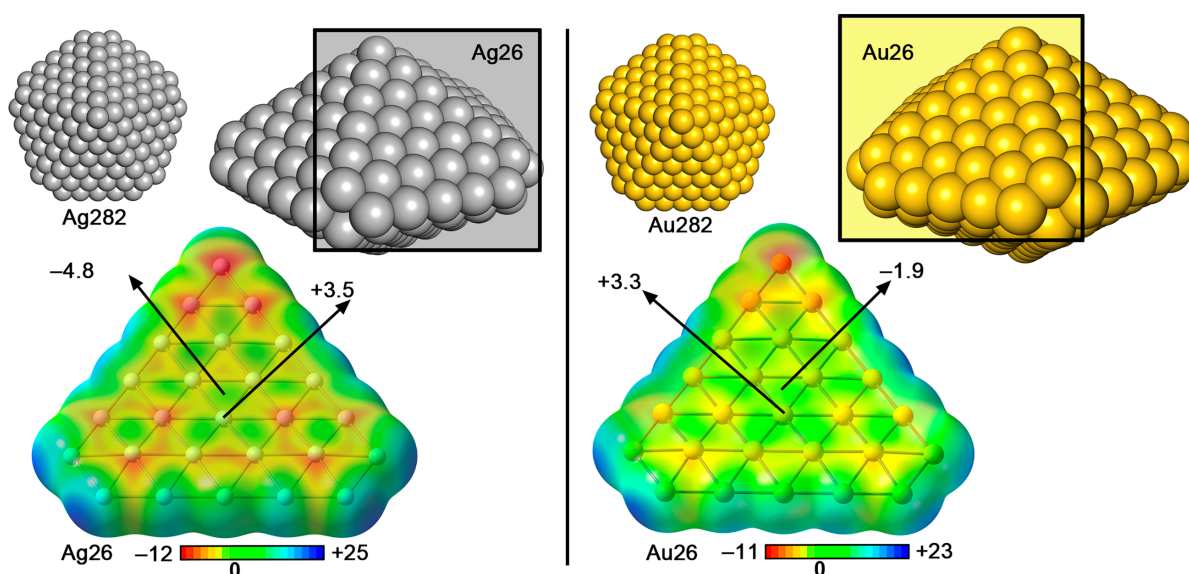
Figure 3. Molecular Electrostatic Potential (MEP) surfaces of Ag26 and Au26 layers. The energy values given at concrete parts of the surface are in kcal/mol (0.002 a.u.).
