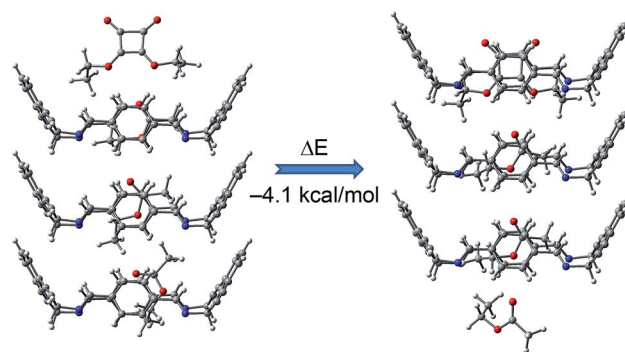
Fig. 8 Favourable energy change due to the substitution of one EtOAc molecule by one diethyl squarate molecule in a minimalist representative channel of \mathbf{3@EtOAc} .
