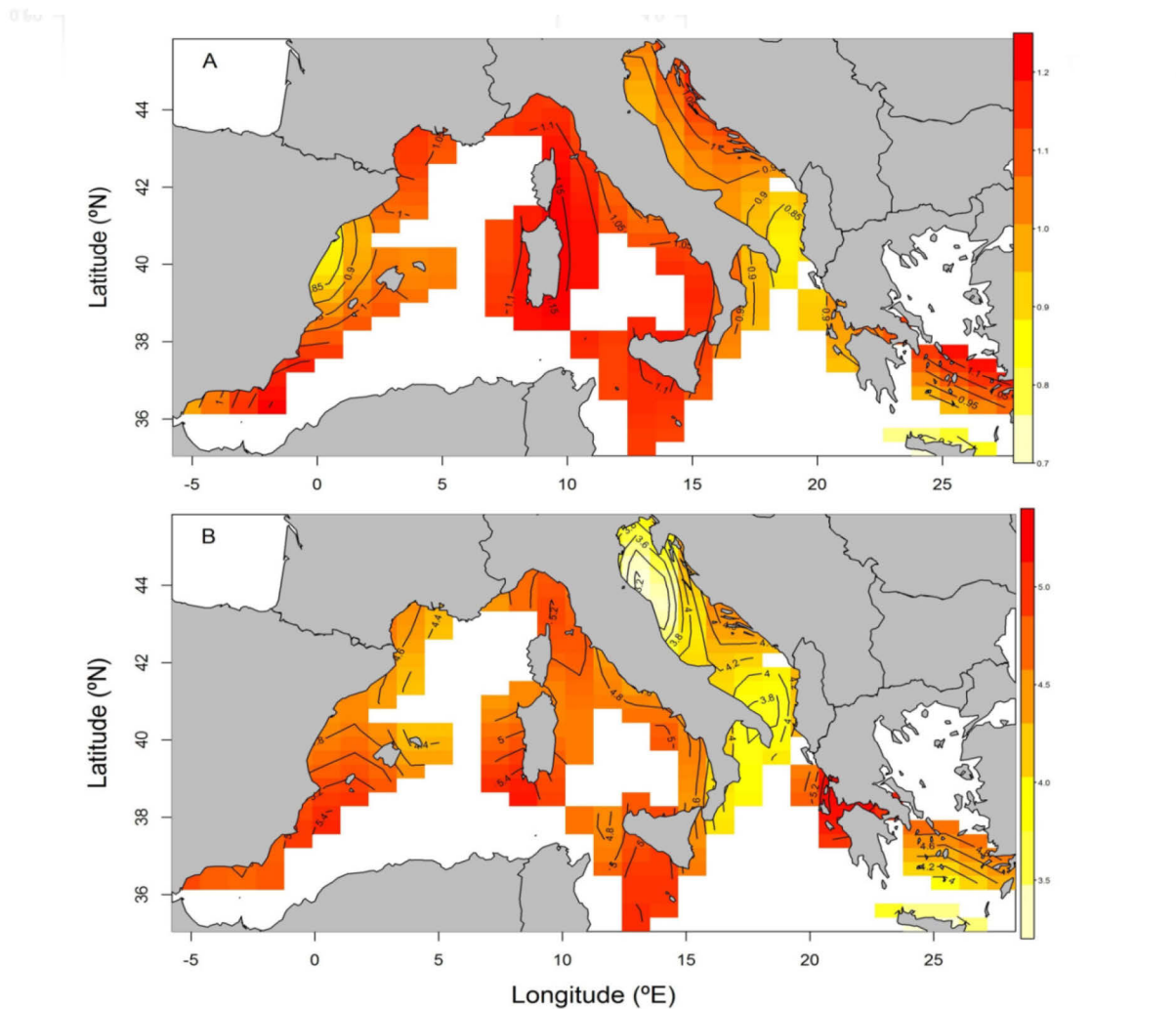
Figure 3.10: Spatial pattern of Shannon diversity H' (A) and species richness S (B) across the Mediterranean Sea as predicted by the GAM model.
