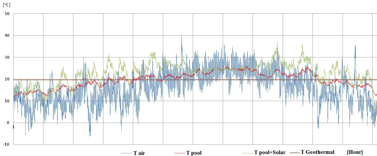
Figure 5 Temperatures of the systems at Balearic Island's. [3][5]
