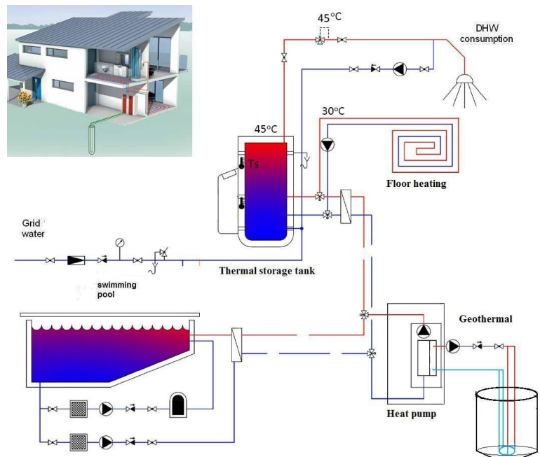
Figure 1. Schematic diagram of a geothermal system with a heat pump [3] [5].
