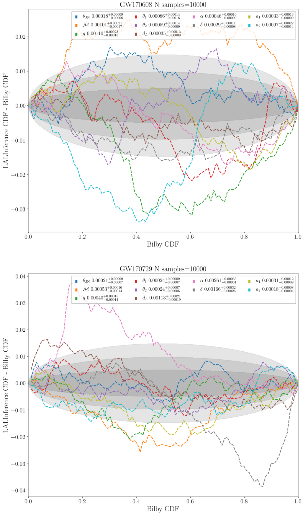
Figure D3. CDF comparison between BILBY and LALINFERENCE for GW170608 and GW170729 .
