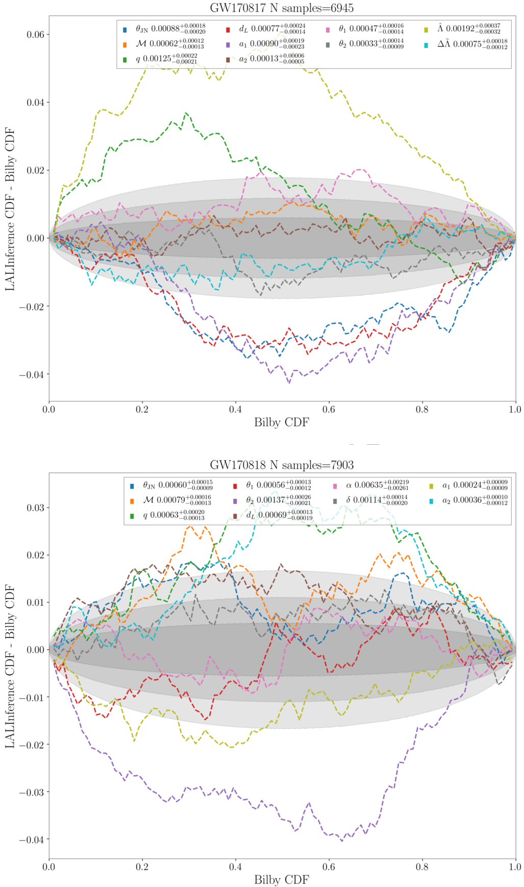
Figure D5. CDF comparison between BILBY and LALINFERENCE for GW170817 and GW170818.
