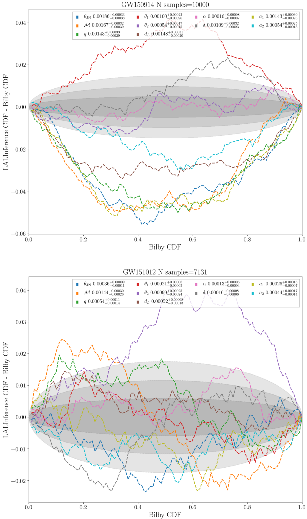
Figure D1. CDF comparison between BILBY and LALINFERENCE for GW150914 and GW151012.
