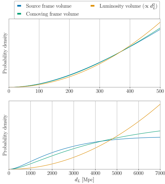
Figure 1. Comparison of distance priors out to redshift z = 0.10 (top panel) and z = 1.02 (bottom panel), respectively corresponding to d_L = 500 Mpc and d_L = 7000 Mpc, according to Ade et al. (2016) cosmology. The upper and lower panels show the range of the luminosity distance priors for the default 128 s and high-mass prior sets, respectively. We display priors that are uniform in luminosity volume, comoving volume, and the (comoving) source frame. The probability density of each curve is normalized with respect to the upper limit cut-off displayed in that panel.
