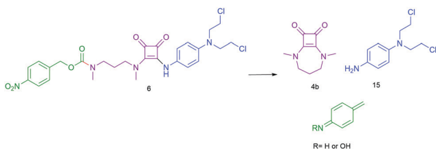
Scheme 1 Self-immolative disassembly of compound 6 triggered by enzymatic reduction of the nitro group.
