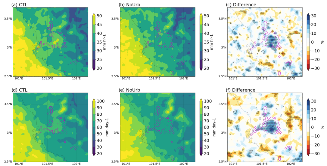
Figure 3. The presence of the city increases heavy rainfall intensities. Mean hourly intensity of events above the 95th percentile for CTL (a) and NoUrb (b) and the percentage difference between CTL and NoUrb runs (c). Mean daily intensity of events above the 95th percentile for CTL (d) and NoUrb (e) and the difference of CTL minus NoUrb runs (f). Urban areas designated in CTL runs are shown with purple contours (c, f) while stippling indicates statistically significant differences using a two-sided Mann–Whitney U test at the 99% confidence level.
