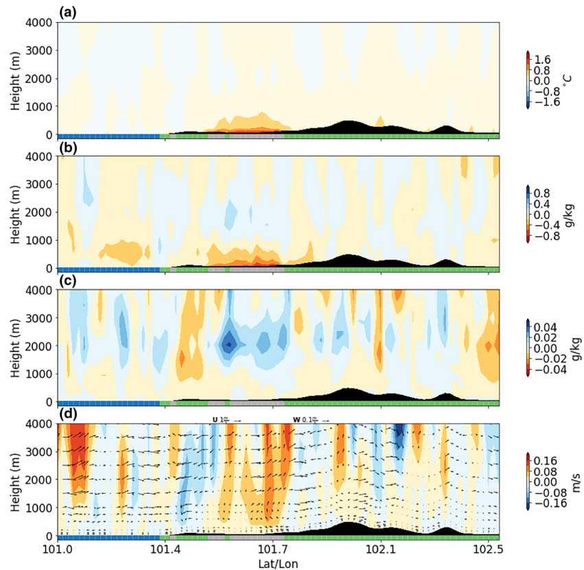
Figure 4. The impact of urban areas on the vertical structure of the atmosphere. Vertical transect along 3.1°N of differences in temperature (a), humidity (b) and cloud water and ice (c), and vertical wind speed (d) between CTL and NoUrb simulations (CTL minus NoUrb) for all hourly rainfall events above the 95th percentile and the preceding 6 hr. Vectors (d) are differences in winds along the cross section between the two experiments. U and W labels indicate the scale of horizontal and vertical wind vectors. The black area represents topography, and the bottom bar shows the ocean (blue), rural (green), and urban (gray) areas in the CTL run.
