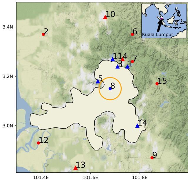
Figure 1. Hourly intensities of extreme rainfall in urban Kuala Lumpur show significant increasing trends, while rural areas are nonsignificant. Spatial distribution of stations showing significant/nonsignificant trends. Urban areas of Kuala Lumpur in 1989 are denoted by the white outlined area. Urban gauges throughout the whole study period 1981–2011 are shown in blue and rural gauges in red, with station ID as number labels (Table S1). Up triangles denote significant increasing trends; dots denote no significant trend. The orange circle shows a 5-km radius circle around one station, used in the urban definition (see section 2.1). The purple point in the inset of Southeast Asia denotes the location of Kuala Lumpur.
