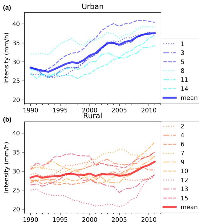
Figure 2. Urban gauges show a more rapid increase in hourly rainfall extremes than rural ones during the last three decades. Ten-year rolling averages of the Q95 of hourly rainfall for (a) each urban station and (b) rural station, and the mean of the gauges. By Q95, we refer to the mean hourly intensity of the declustered events above the 0.95 quantile. See Figure 1 in the main text and Table S1 for locations and other station information. The station IDs are shown in the legend.
