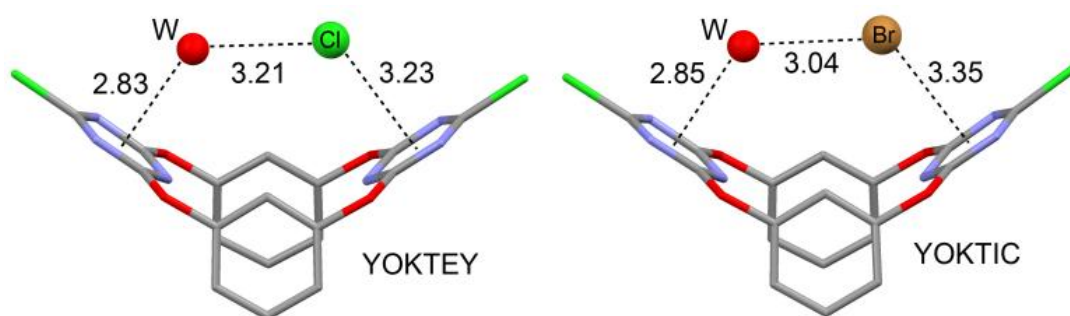
Figure 1.42. X-ray crystal structures of the complexes between tetraoxacalix[2]arene[2]triazine hosts and chloride (left) and bromide (right), with distances in Å. 213 The CSD reference codes are indicated.
