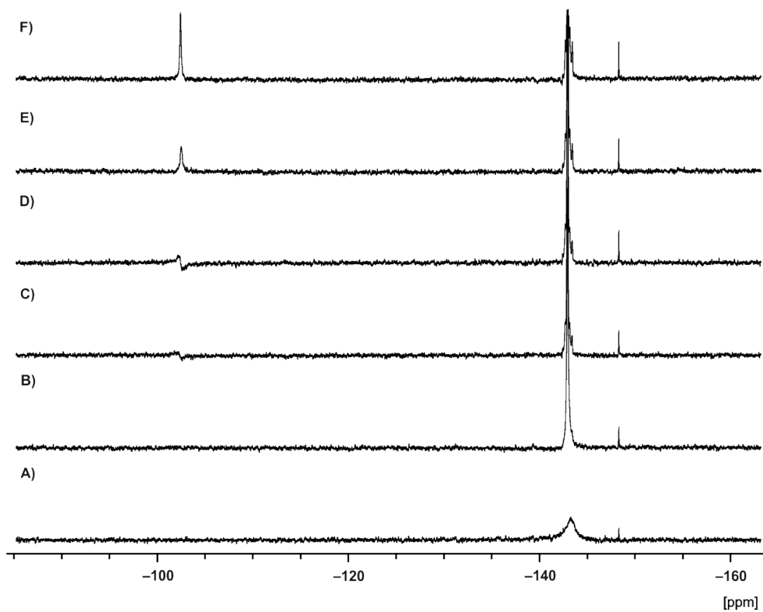
Figure 3.11. Selected expansion of ^{19}\text{F} -NMR spectra obtained during the titration of receptor 2 in DMSO with TBAF· 3\text{H}_2\text{O} at 298 K. A) 2 + 1.8 eq. of TBAF· 3\text{H}_2\text{O} . B) 2 + 3.1 eq. of TBAF· 3\text{H}_2\text{O} . C) 2 + 4.03 eq. of TBAF· 3\text{H}_2\text{O} . D) 2 + 4.7 eq. of TBAF· 3\text{H}_2\text{O} . E) 2 + 5.3 eq. of TBAF· 3\text{H}_2\text{O} . F) 2 + 6.3 eq. of TBAF· 3\text{H}_2\text{O} . [\mathbf{2}] = 1 \text{ mM} .
