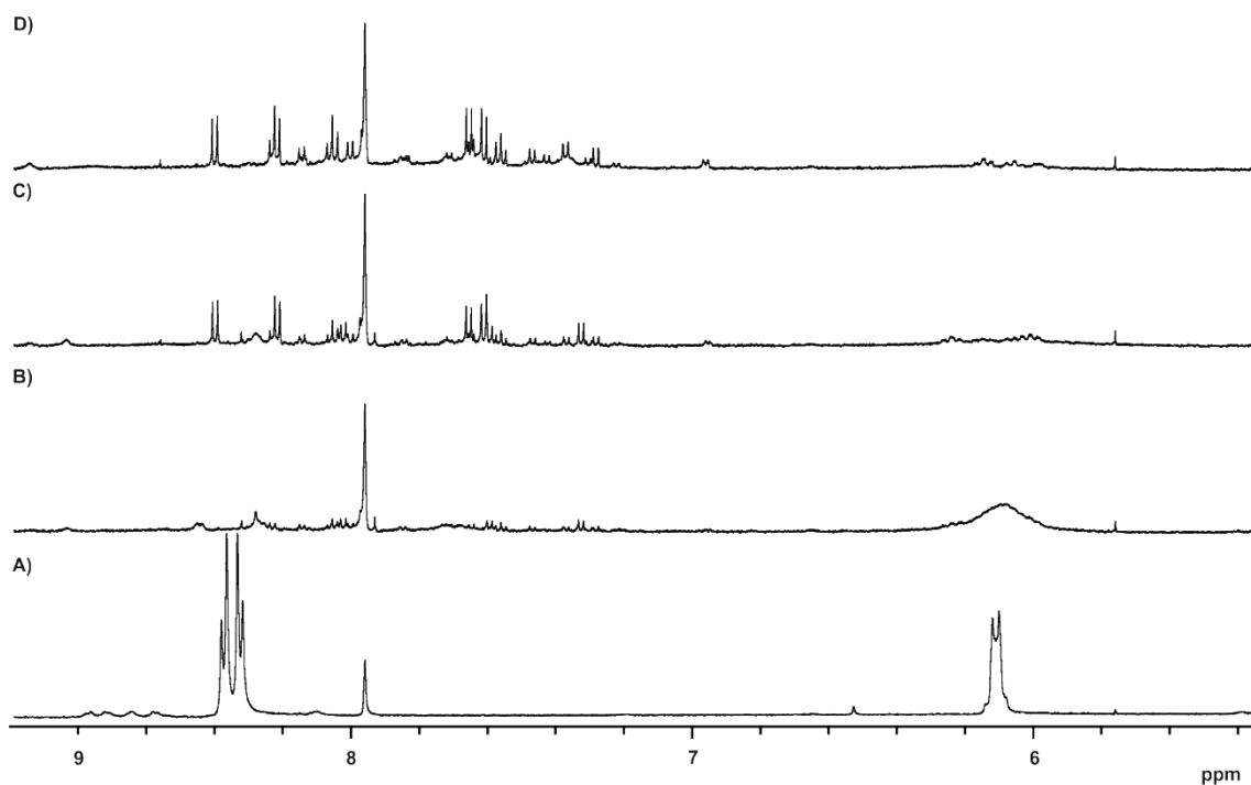
Figure 3.10. Selected expansion of ^1\text{H} -NMR spectra obtained during the titration of receptor 2 in DMSO with TBAF· 3\text{H}_2\text{O} at 298 K. A) 2 . B) 2 + 1.8 eq. of TBAF· 3\text{H}_2\text{O} . C) 2 + 3.1 eq. of TBAF· 3\text{H}_2\text{O} . D) 2 + 8.2 eq. of TBAF· 3\text{H}_2\text{O} . See Figure 3.2 for proton assignment. [\mathbf{2}] = 1 \text{ mM} .
